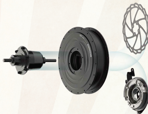
IMA2 REAR HUB MOTOR
